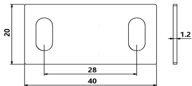
TY-Square iron sheet
